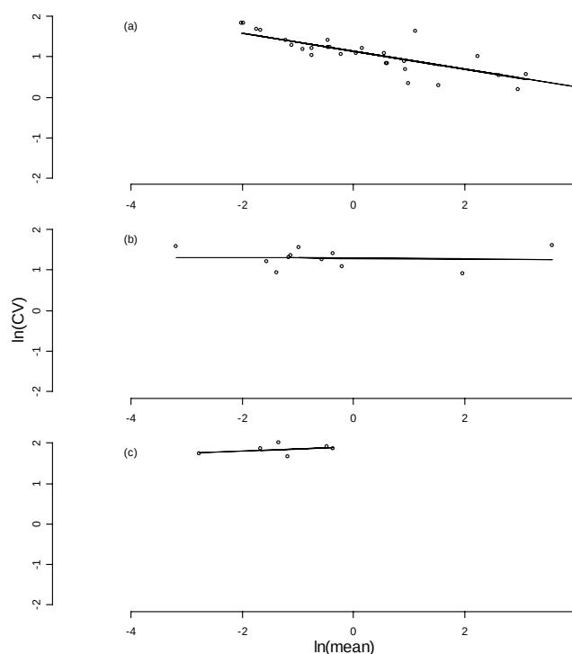
Figure 4. Taylor power plot of the \ln transformed coefficient of variation (CV) for the annual age-0 index versus its mean. The CV was estimated according to eq. 1. Panel (a) is KC, (b) is NSe and (c) NSs.
