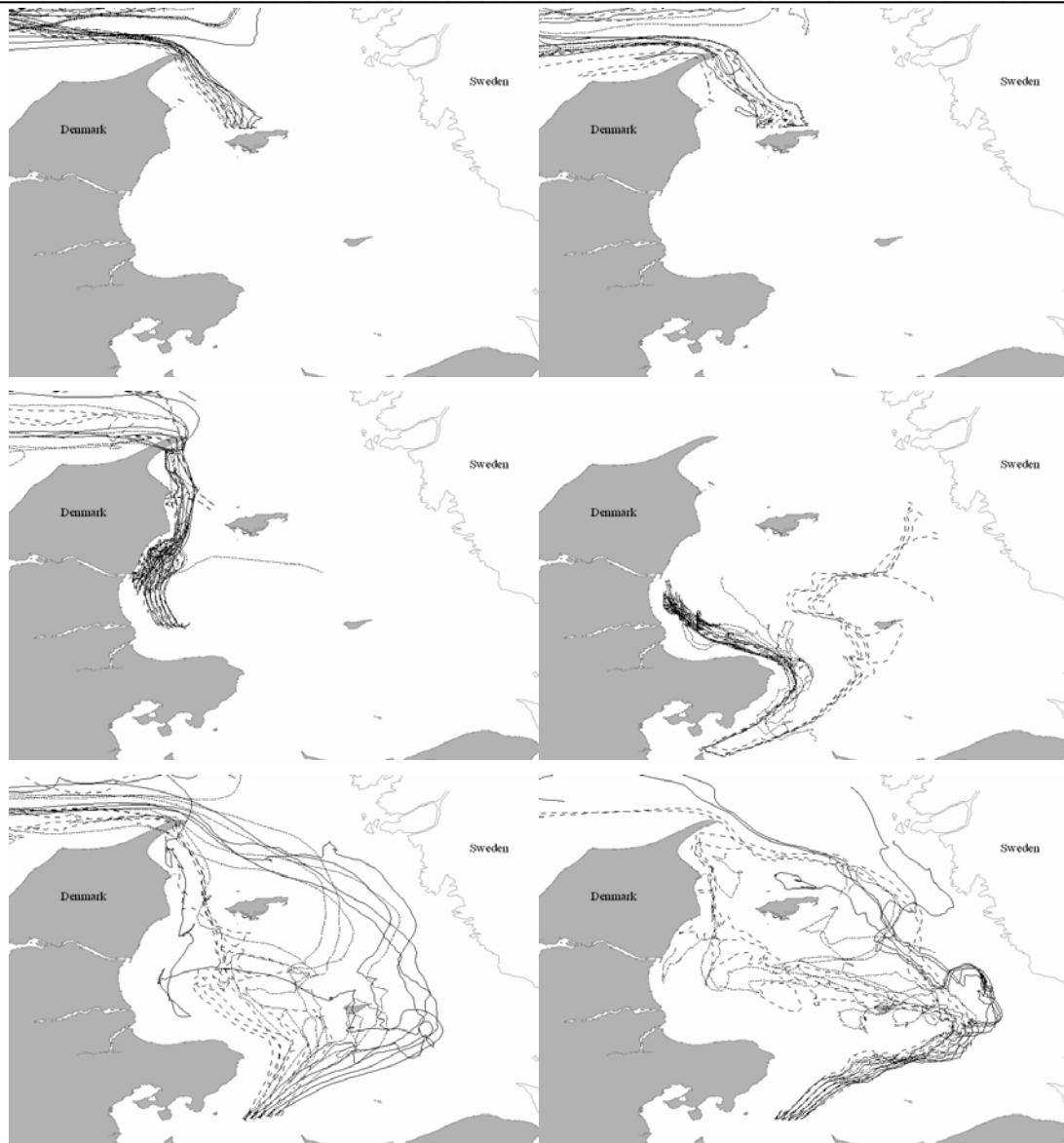
Figure 7. Each map shows drift trajectories for 5 drifters released in 1988. Top panel is drifters released at the northern spawning size, middle panel is drifters from the middle spawning site and bottom panel is drifters released at the southern spawning area. Figures in left column are drifters released at depth 1, 3 and 5 m shown by fine dashed, coarse dashed and solid line, respectively. Figures in the right column are drifters released at 7, 9 and 11 m, shown by fine dashed, coarse dashed and solid line, respectively.
